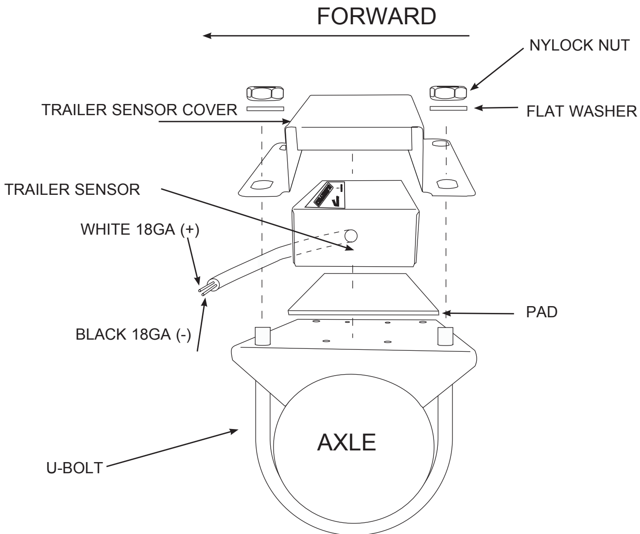
Figure 1: Side view of sensor assembly mounted on the axle.
