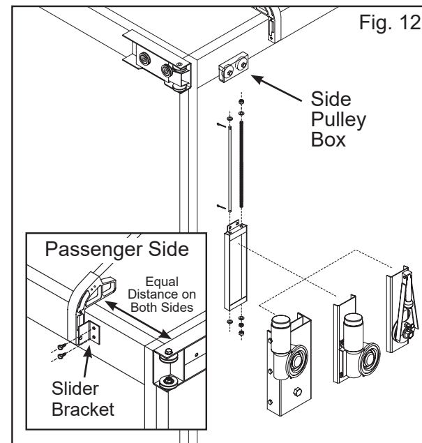
Side Mount
