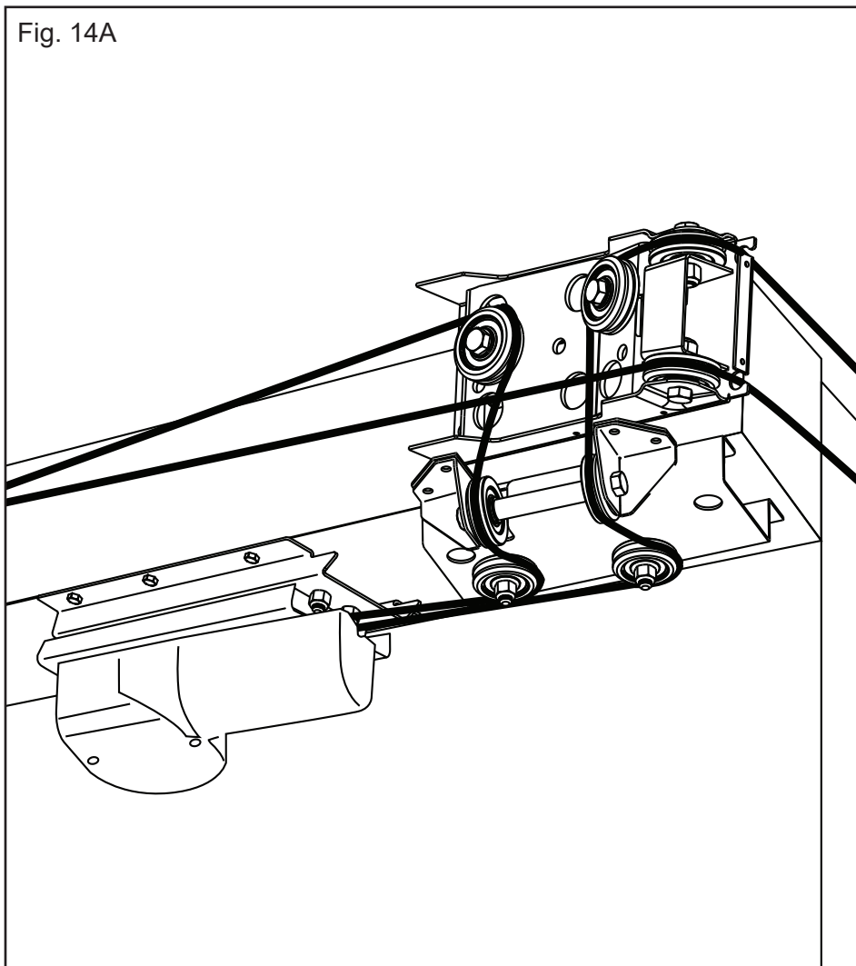
Horizontal Motor Mount / 502-0630
