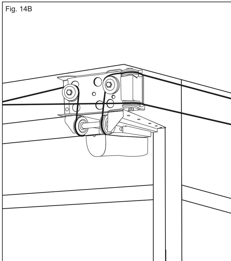
Horizontal Motor Mount / 502-0361
