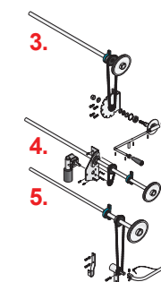
Twin Cable Top Slider
