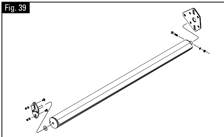
Electric Core System & Roller Tube Assembly (Fig. 39).
